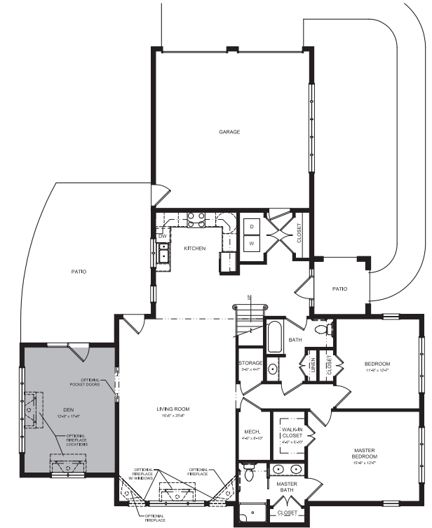
Configuration Three 1,752 SQ FT
